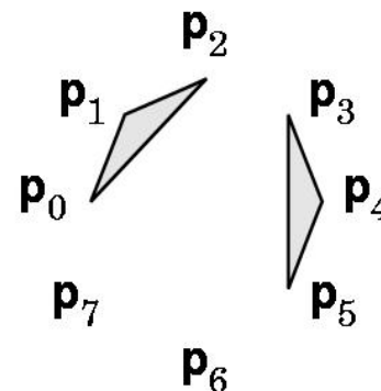
GL_TRIANGLES
