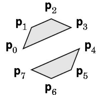
GL_QUADS
