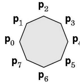
GL_POLYGON
