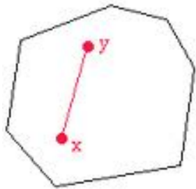
A convex polygon
