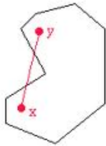
A non-convex polygon
